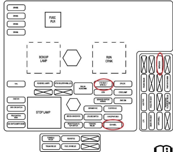
CG fuse panel in passenger footwell
