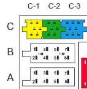
Fig. 3 Radio Connectors
