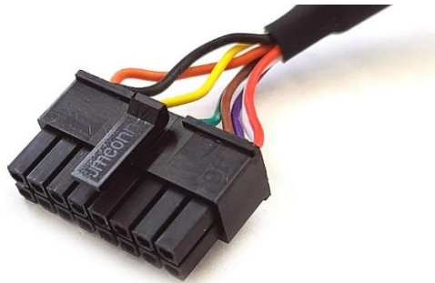
Fig. 5 16-pin plug
